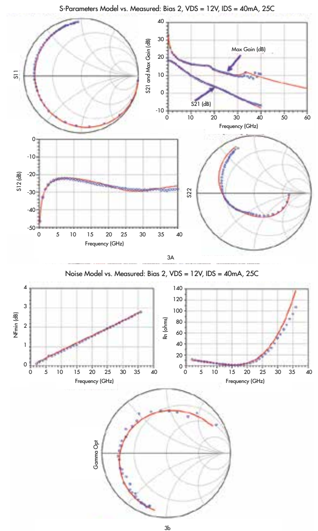
3. This figure illustrates the 0.2-to-40 GHz S-parameter (a) and 2-to-36 GHz noise model (b) performance for the TGF2942 small-signal model (HMT-QOR-TGF2942-SS-001). The parameters are as follows: Vds = 12 V, Ids = 40 mA, 25°C, 50-Ω Smith charts. The solid red lines represent model data, while the blue circles represent measured data.
