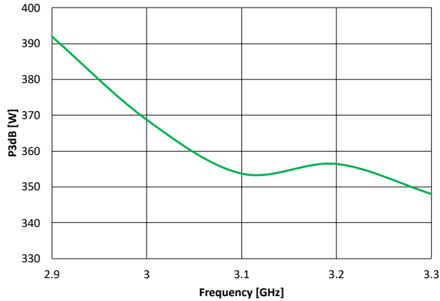
P3dB vs. Frequency at 25 °C
