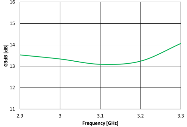
G3dB vs. Frequency at 25 °C
