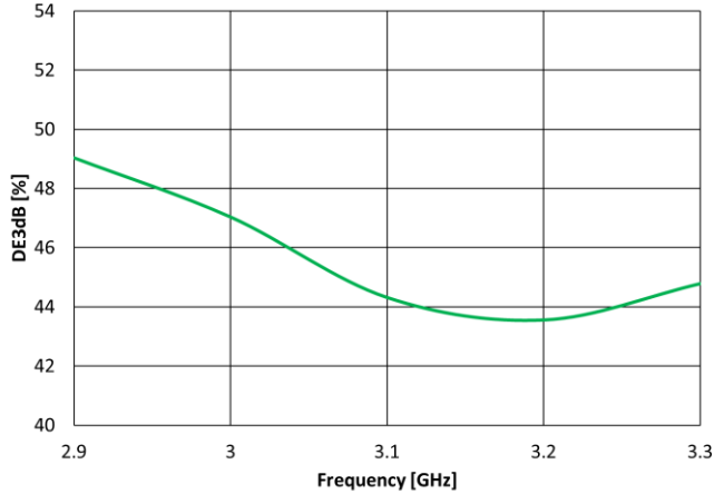
DE3dB vs. Frequency at 25 °C
