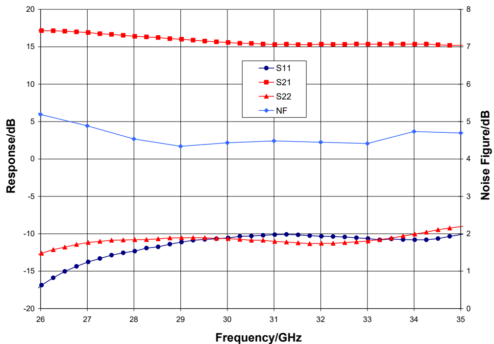
Narrow-band Performance, V_{dd1} = V_{dd2} = 5.0 V, I_{dd1} = I_{dd2} = 45 mA, T_A = 25 °C
