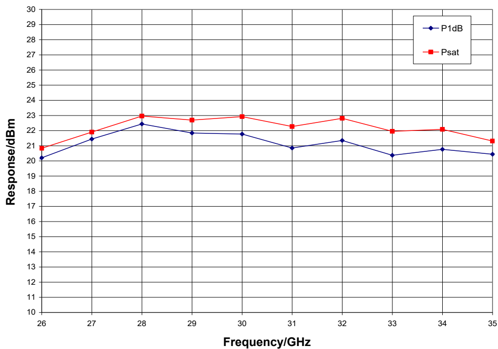
Output Power, V_{dd1} = V_{dd2} = 5.0 \text{ V} , T_A = 25 \text{ }^{\circ}\text{C}
