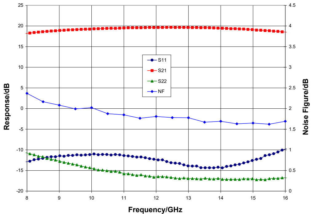
Narrow-band Performance, V_{dd} = 3.0\text{ V} , T_A = 25\text{ }^\circ\text{C}
