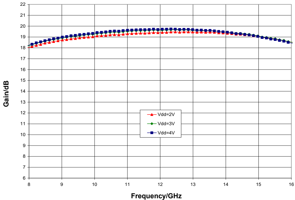
Gain vs. V_{dd} , T_A = 25\text{ }^\circ\text{C}
