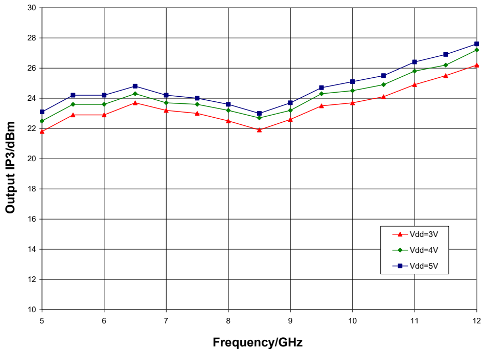
Output IP3 vs. V_{dd} , T_A = 25\text{ °C}
