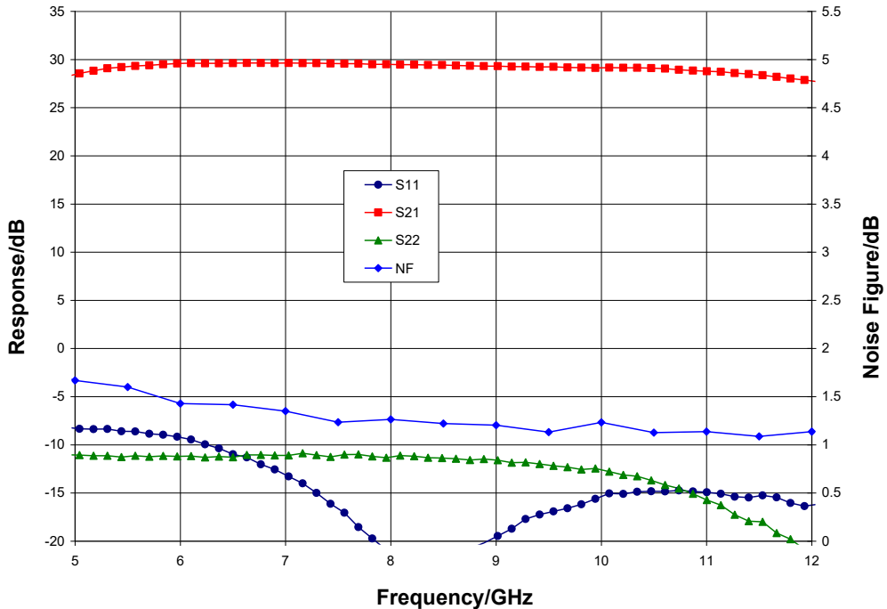
Narrow-band Performance, V_{dd} = 4.0\text{ V} , T_A = 25\text{ }^\circ\text{C}
