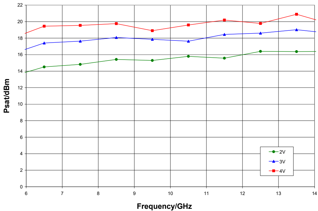
Psat vs. V_{dd} , V_{gg} = 1.5\text{ V} , T_A = 25\text{ }^\circ\text{C}
