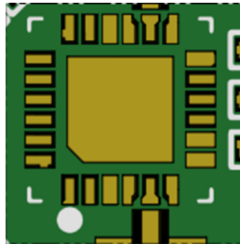
Landing Pattern
