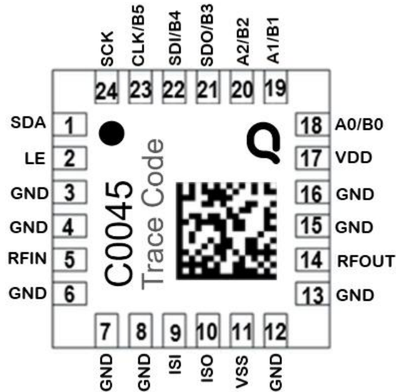
Top view of package base
