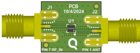
Figure 2a. QPQ5604 Evaluation Board PCB
