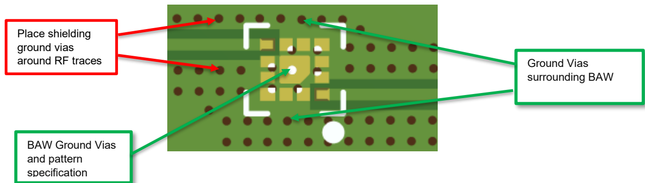
Figure 4. Recommended 10-Via count GND via Pattern
