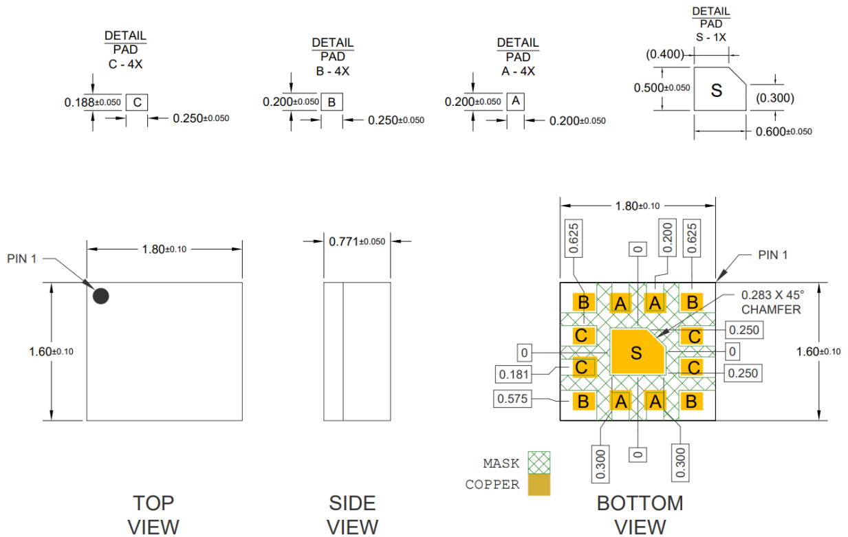
Figure 6a. Marking Diagram
