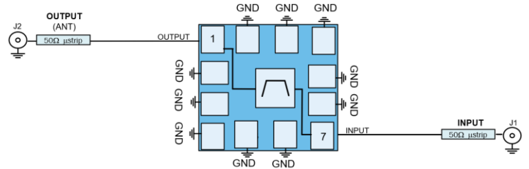
Figure 2b. QPQ5604 Evaluation Board Schematic
