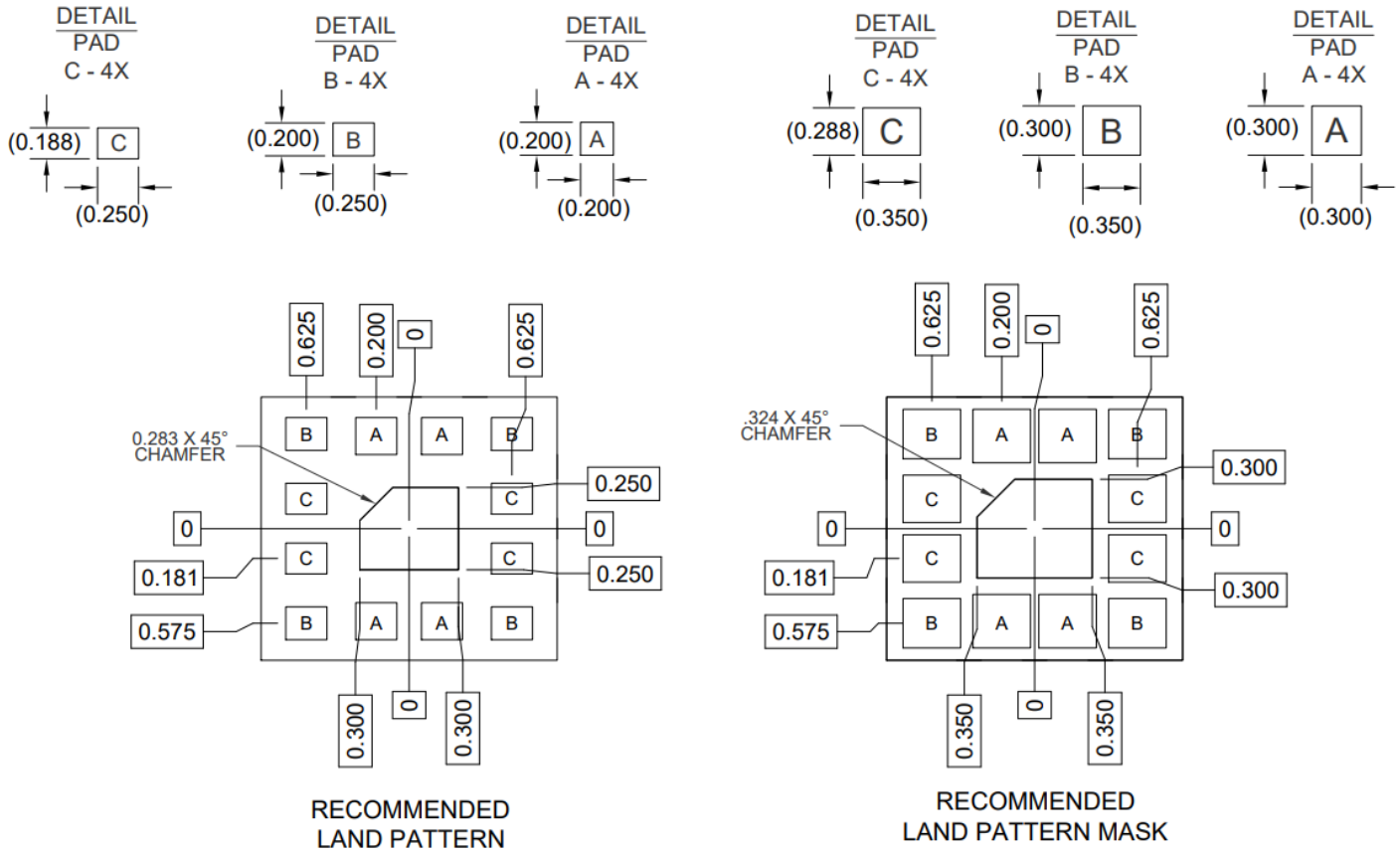
Figure 5a. PCB Footprint Recommended Landing Pattern
