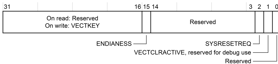
Figure 30-23. AIRCR
