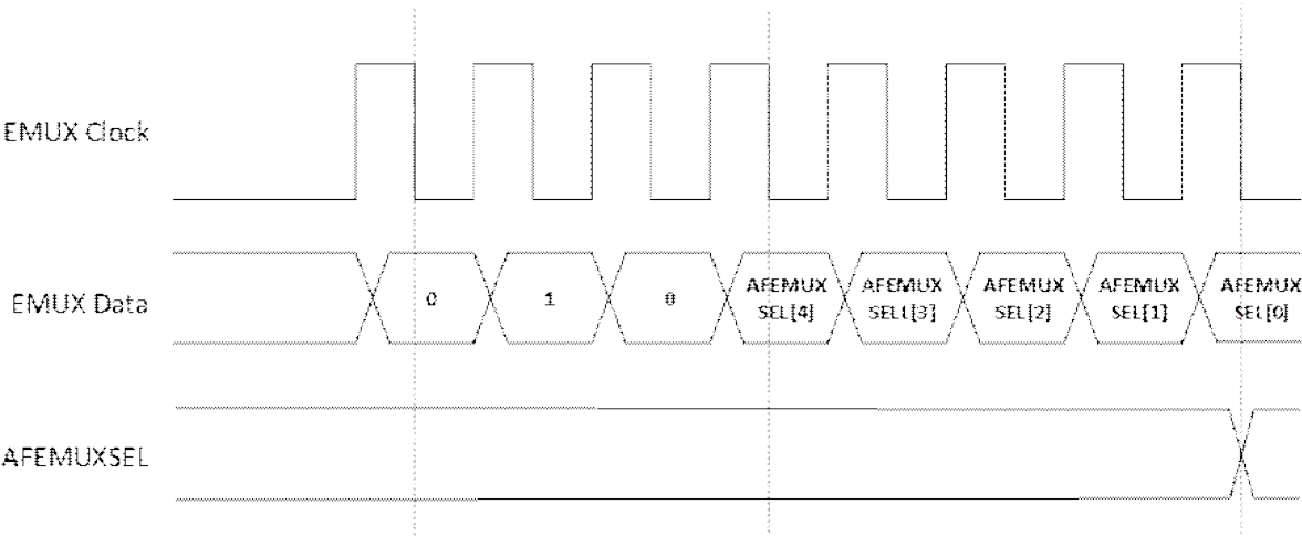
Figure 23-1. EMUX Timing Diagram
