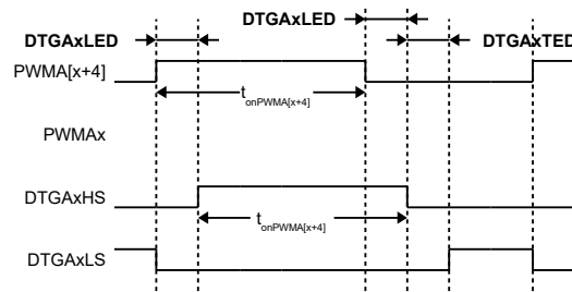
Figure 12-7. DTGAx LED and TED with On Time Preservation Example
