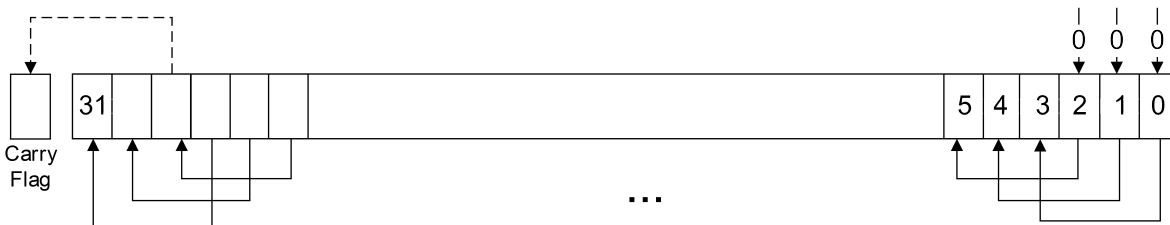
Figure 30-14. LSL #3
