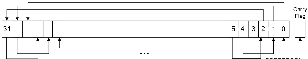
Figure 30-15. ROR #3
