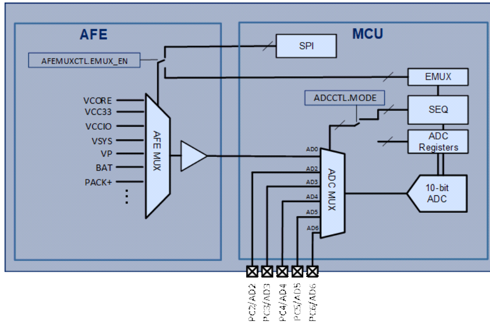
Figure 22-1. ADC MUX inputs
