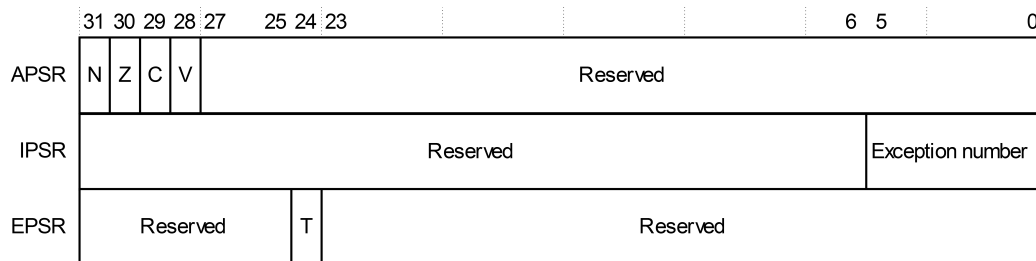
Figure 30-3. PSR
