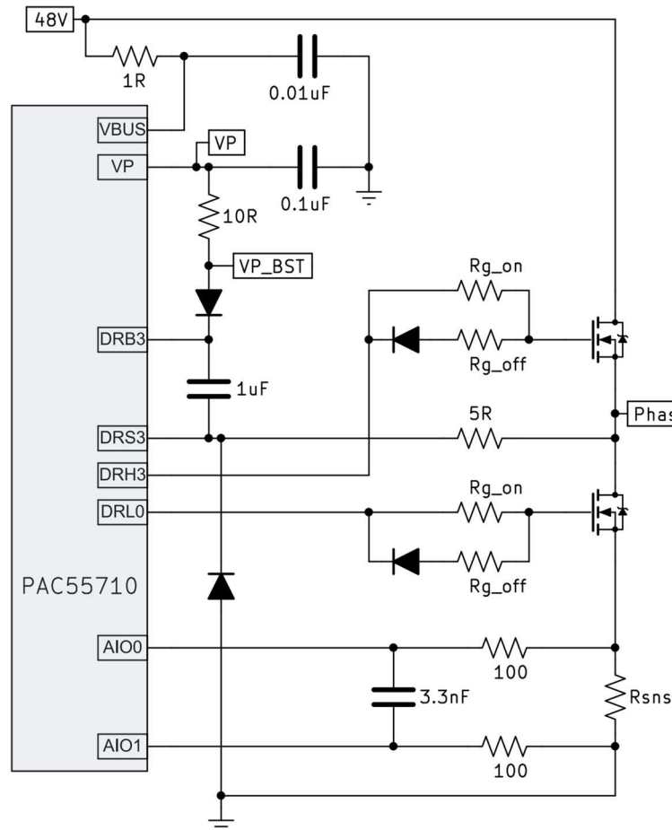
Fig. 4-4. Phase U of inverter drive with PAC55710
