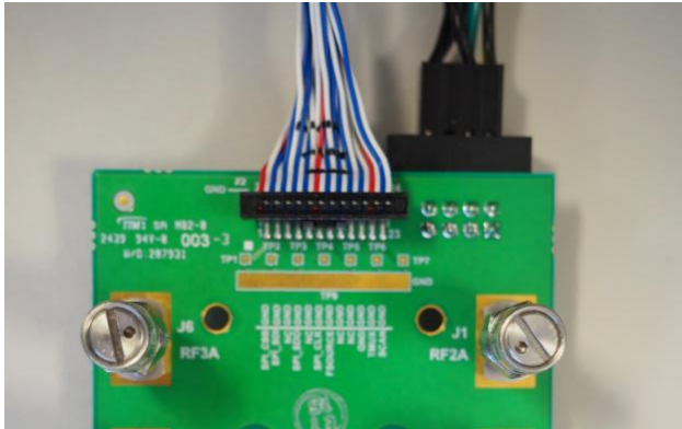
Figure 17: Bottom side view: IO cable connected to X2
